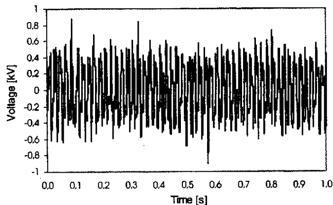
Figure 8. Voltage waveform at the Arc Furnace (Bus 7)
