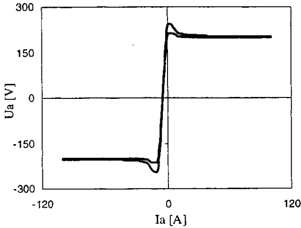
Figure 1. Arc furnace voltage-current characteristic
