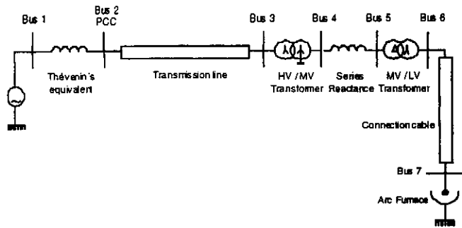
Figure 2. Electrical network supplying the arc furnace
