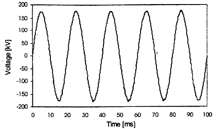
Figure 3. Voltage waveform at the PCC (Bus 2)
