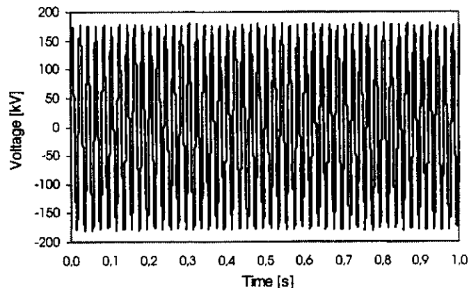
Figure 7. Voltage waveform at the PCC (Bus 2)
