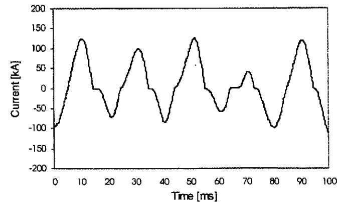
Figure 6. Current waveform at the Arc Furnace (Bus7)
