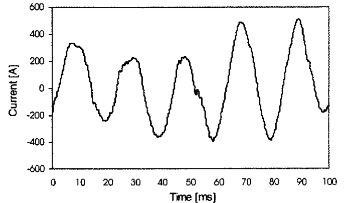
Figure 4. Current waveform at the PCC (Bus 2)
