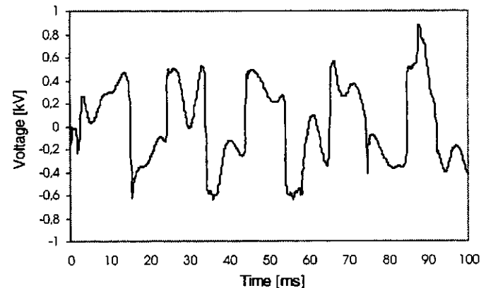
Figure 5. Voltage waveform at the Arc Furnace (Bus7)
