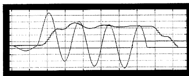
Fig.12. Sample test results for the relay of Fig.8 tested in the simple system of Fig.11 (phase A current, its magnitude as measured by the relay and the TRIP signal).
