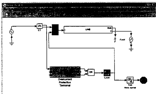
Fig.11. Closed-loop test of the relay of Fig.8 in a simple power system model.
