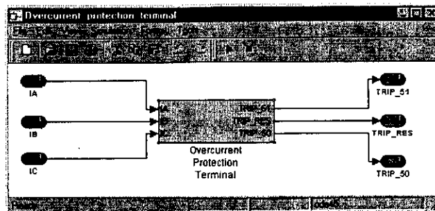
Fig.8. Overcurrent relay model (IA, IB, IC - input currents, TRIP_51, TRIP_50, TRIP_RES - targets).
