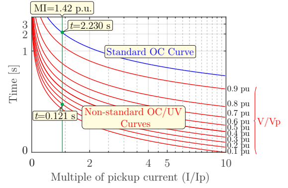
Fig. 3. Practical illustration of tripping characteristics.
