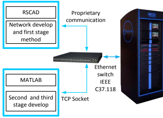
Fig. 5. Software in the loop (SiL) scheme using an RTDS, Transmission Control Protocol socket, LAN switch and external PC.
