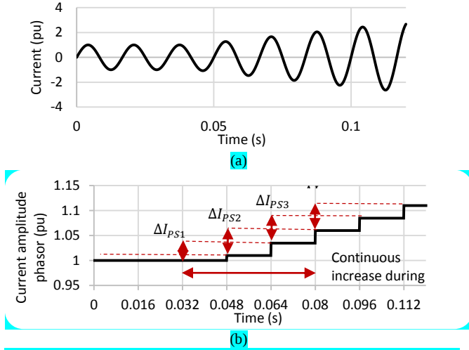
Fig. 3. Stable power swing (a) current signal and, (b) current phasor amplitude in both in pu.
