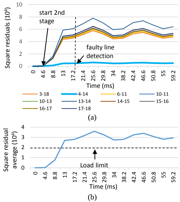
Fig. 10. Area 4, lines square residuals during an AB fault at 65% of line 4-14, (a) sum of squared residuals in all the suspected lines and (b) average between the lines maximum and minimum sum of square residuals.
