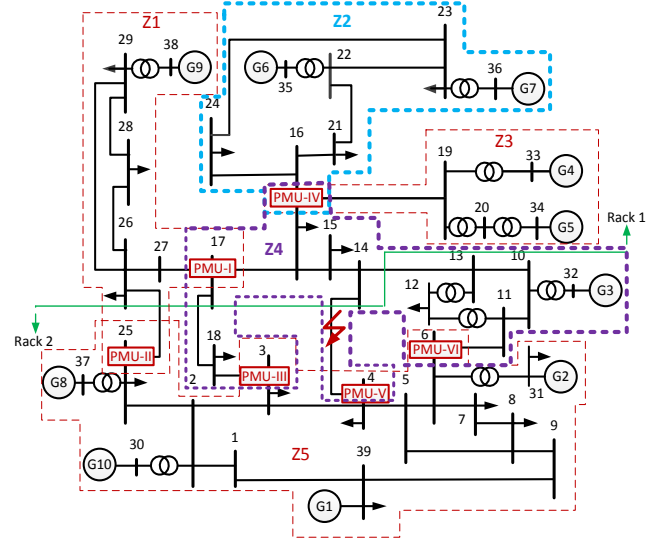
Fig. 6. IEEE 39 bus system with PMUs and the area partitioned.
