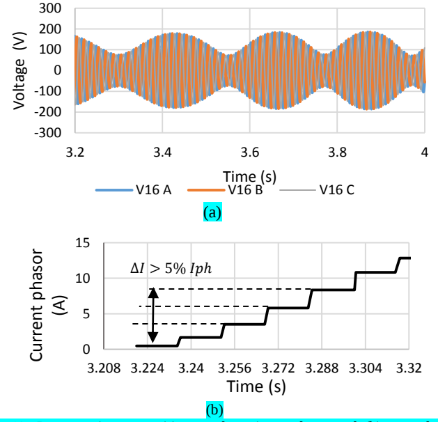
Fig. 12. Power swing case, (a) secondary time voltage and (b) secondary current phasor zoom-in.
