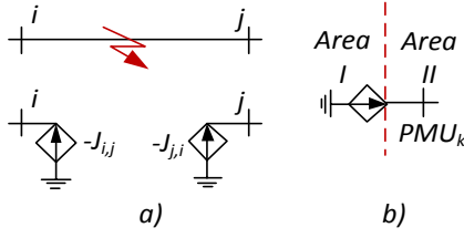
Fig. 4. Elements substitutions, a) transmission line and b) PMU between two areas.
