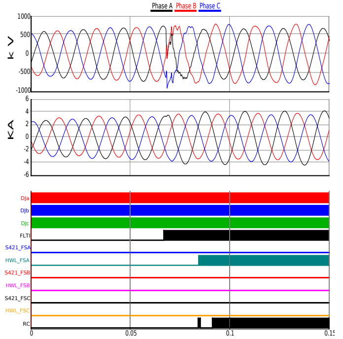
Fig. 6. Oscillography for phase A to ground fault (AG) and week infeed condition. R_f = 200 \Omega .
