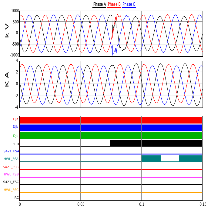
Fig. 7. Oscillography for phase A to ground fault (AG) and very week infeed condition. R_f = 200 \Omega .
